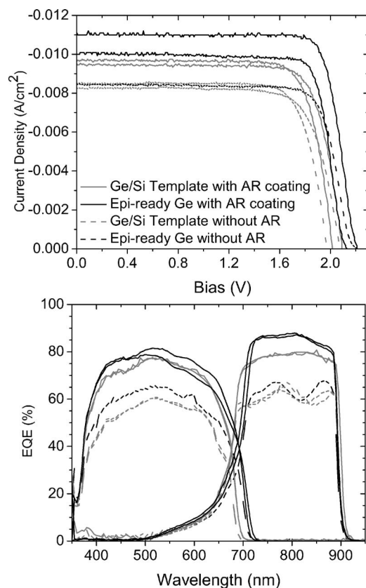
FIG. 4. Photovoltaic I - V curves (top) and spectral response (bottom) for the GaInP/GaAs solar cells grown on Ge/Si epitaxial templates and on a bulk epi-ready Ge substrate.
