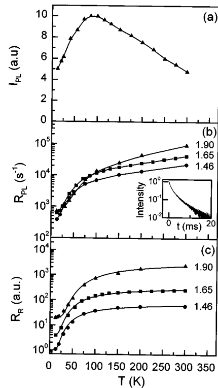
FIG. 2. (a) Temperature dependence of the integrated photoluminescence intensity, I_{\text{PL}} , of Si nanocrystals in SiO 2 . (b) Temperature dependence of the photoluminescence decay rate, R_{\text{PL}} , measured at emission energies of 1.46, 1.65, and 1.90 eV. The inset shows a typical decay trace taken at 1.65 eV and 15 K. (c) Temperature dependence of the radiative rate at emission energies of 1.46, 1.65, and 1.90 eV, obtained from a multiplication of the temperature dependent I_{\text{PL}} data in (a) and R_{\text{PL}} data in (b). The solid curves are best fits of R_R using a model that takes into account the exchange splitting of the energy levels of quantum-confined excitons in the Si nanocrystals.
