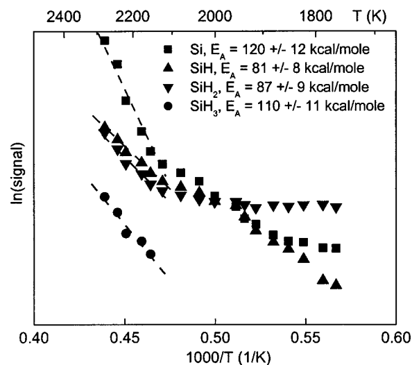
FIG. 3. SiH x radical signals measured from an aged W wire at a total pressure of 5 \times 10^{-6} Torr. Activation energies quoted are accurate to within \pm 10\% , due to uncertainties ( \pm 50 K) in wire temperature; error bars are not shown.
