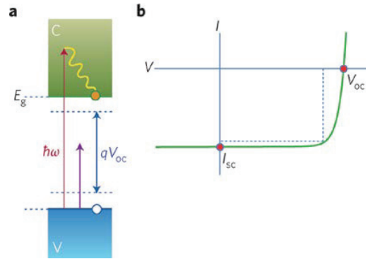
Fig. 1. a , Energy diagram of a single-junction solar cell. Light at energy \hbar\omega (red arrow) creates an excitation from the valence ( V ) to the conduction ( C ) band of a semiconductor. After thermalization in the conduction band an electron–hole pair is formed across the bandgap with energy E_g . Light with energy below the bandgap (purple arrow) is not absorbed. b , Typical current–voltage ( I – V ) characteristics of a solar cell. The short-circuit current I_{sc} is a direct measure of the conversion efficiency from incident photons to electrical current. The open-circuit voltage V_{oc} is lower than E_g due to entropic reasons. The dashed lines indicate the maximum-power operating point of the solar cell.
