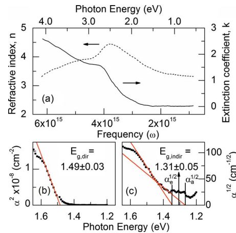
FIG. 3. (Color online) Spectroscopic ellipsometric analysis of Br 2 -etched Zn 3 P 2 wafers at 295 K showing: (a) the derived n(\omega) , k(\omega) data in the spectral range 0.5–4.0 eV; (b) the test of \alpha(\omega) for direct transitions; and (c) the test of \alpha(\omega) for indirect transitions.
