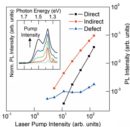
FIG. 2. (Color online) Relative intensities of the direct gap, indirect gap, and defect-assisted PL of Br 2 -etched Zn 3 P 2 wafers as a function of laser pump intensity at 295 K. The inset shows the normalized PL spectra across the same range of laser pump intensities.
