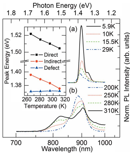
FIG. 1. (Color online) Normalized PL spectra of Br 2 -etched Zn 3 P 2 wafers in the temperature ranges (a) 5.9–29 K and (b) 200–310 K. The inset shows the energies, as a function of temperature, of the direct and indirect interband transitions, as well as a defect-assisted transition.
