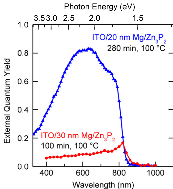
Figure 2. External quantum yield observed in ITO/Mg/Zn 3 P 2 solar cells with different Mg layer thicknesses after annealing at 100 °C in air. Devices with thinner 20 nm Mg layers (blue) show high external quantum yield, but devices with thicker 30 nm Mg layers (red) show reduced external quantum yield.
