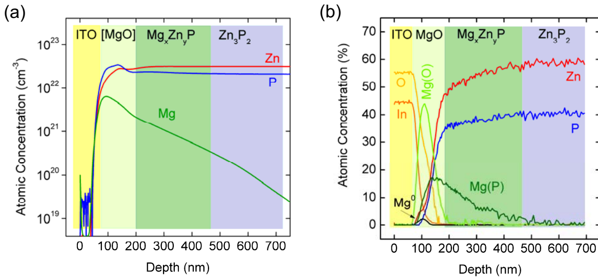
Figure 3. Composition profiling of ITO/Mg/Zn 3 P 2 solar cells by (a) secondary ion mass spectrometry (SIMS) and (b) x-ray photoelectron spectroscopy (XPS) after annealing at 100 °C for 72 hours in air. The data show layers corresponding to ITO (yellow), MgO (light green), Mg x Zn y P (dark green) and Mg-doped Zn 3 P 2 (light blue). Mg metal reacts to form both MgO and Mg x Zn y P at the junction of ITO/Mg/Zn 3 P 2 solar cells.
