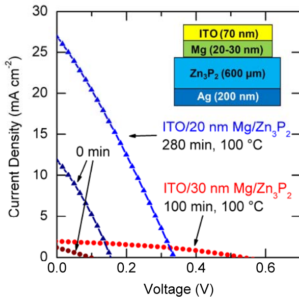
Figure 1. Photovoltaic performance under simulated AM1.5 illumination observed in ITO/Mg/Zn 3 P 2 solar cells. Red traces show annealed devices with 30 nm Mg layer, where dark red corresponds to the as-fabricated device; and blue traces show annealed devices with 20 nm Mg layer, where dark blue corresponds to the as-fabricated device.
