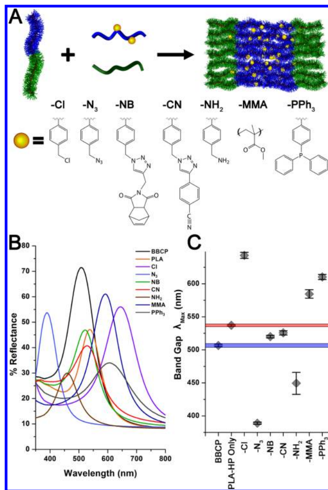
Figure 4. (A) Modifying a PS homopolymer with additional functional groups (yellow spheres) allows this random copolymer to act as a “Trojan horse” to bring these functional groups into the BCCP array. (B) All BCCP/RCP blends generated well-ordered arrays with clear photonic band gaps; the amount of reflection varied as a function of sample thickness and degree of disorder within the sample, but the quality of the lamellar arrays remained mostly unchanged. (C) The photonic band gap \lambda_{\max} values (measured in triplicate) of the RCP blends do not overlap with either the BCCP \lambda_{\max} (blue region) or PLA-HP-only \lambda_{\max} (red region) controls, indicating that the RCPs were indeed incorporated into the arrays. All blended samples contained \sim 25 wt% each PLA-HP and RCP, with the exception of the BCCP-only control, the PLA-only control (which contained the same amount of BCCP and PLA-HP as the others but no RCP), and PPh 3 , which was 12.5 wt% each PLA-HP and RCP.
