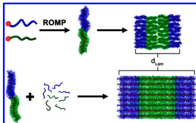
Figure 1. Brush block copolymers generated from norbornene-terminated polystyrene (PS) and poly(lactic acid) (PLA) macromonomers adopt rigid rod-like conformations that allow them to form lamellar arrays with large periodicities. Adding small PS and PLA homopolymers swells these arrays, increasing their domain spacing.
